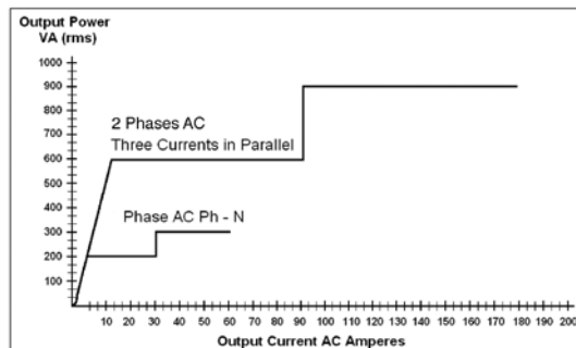
Figure 13 Current Output Power Curve
