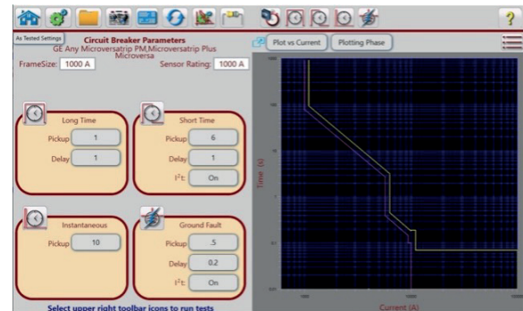
Figure 7: GE microversatstrip curves
